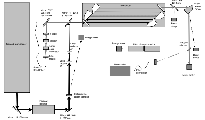
Figure 1. Experimental layout.
